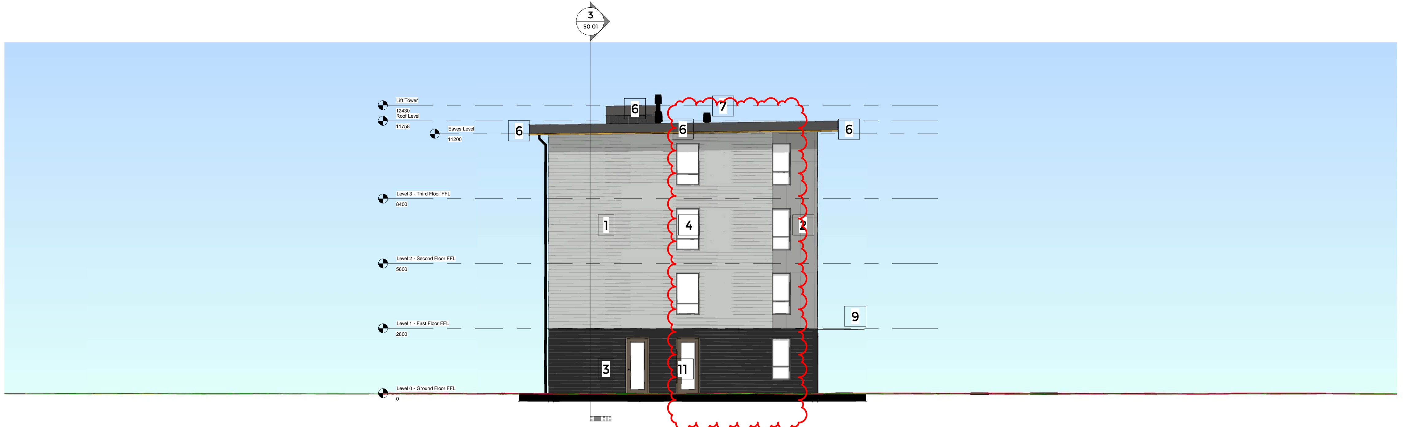
1 South Elevation 1:100
