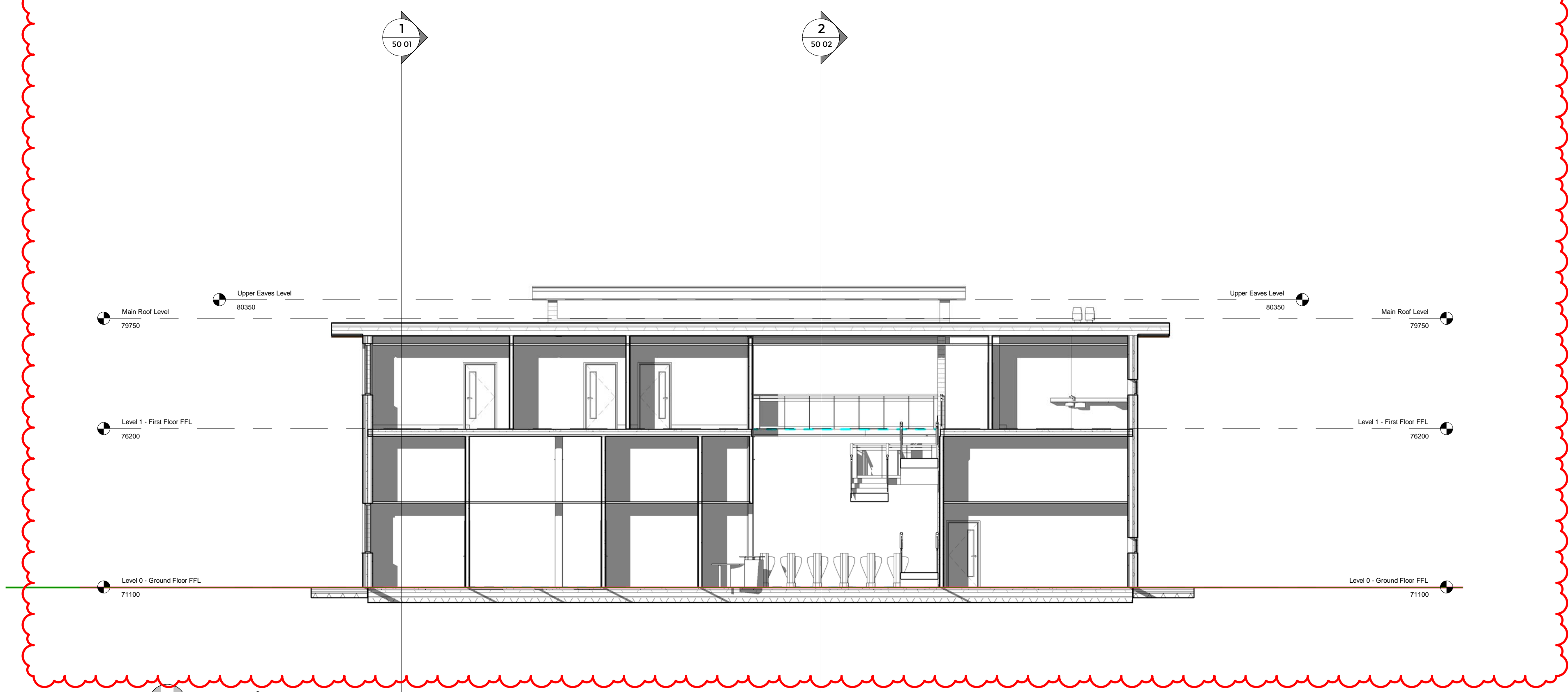
2 Section 2 1:100
