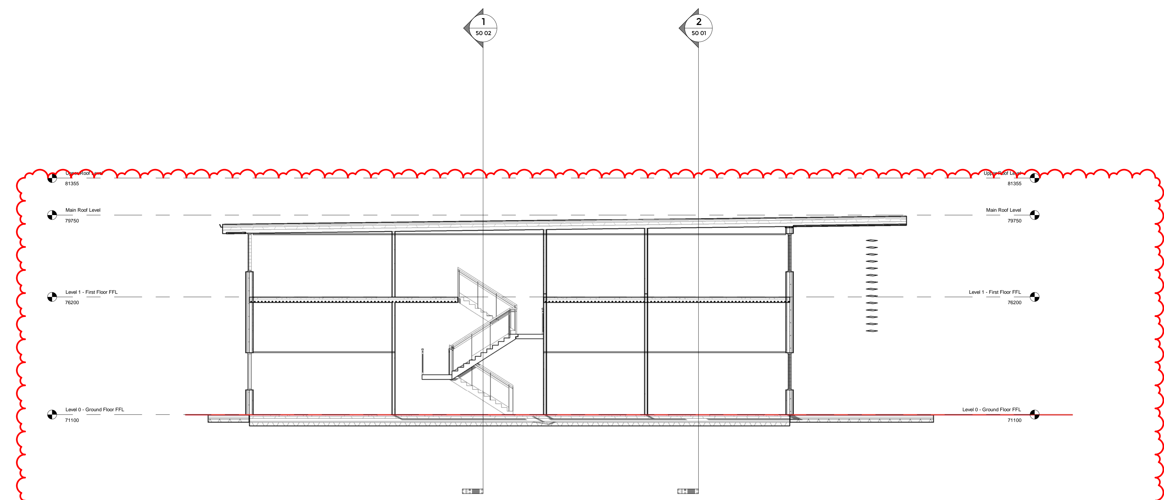
1 Section 1 1:100
