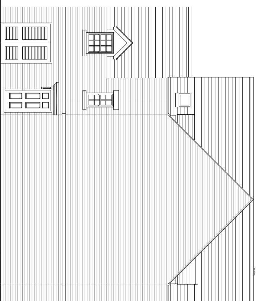
COURTYARD ELEVATION
