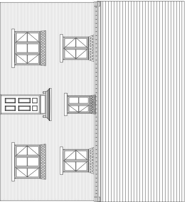
FRONT ELEVATION
