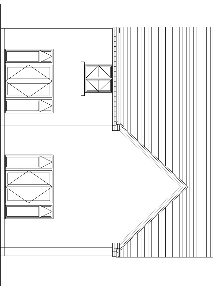
REAR ELEVATION
