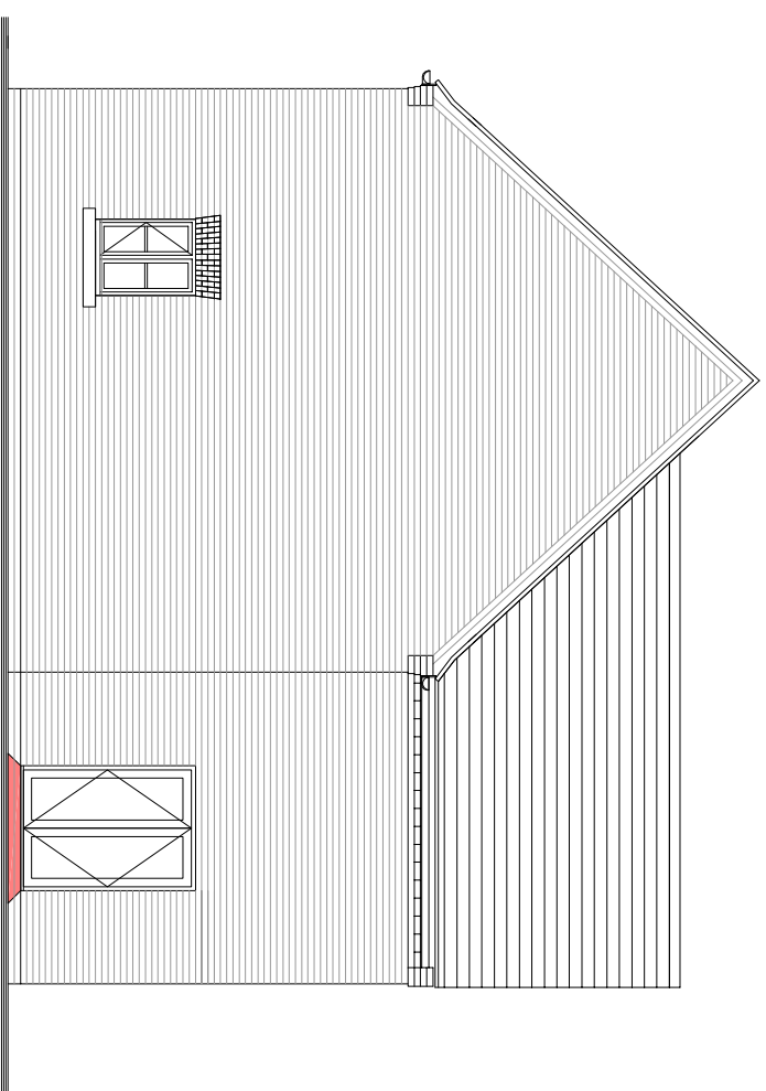
SIDE ELEVATION
