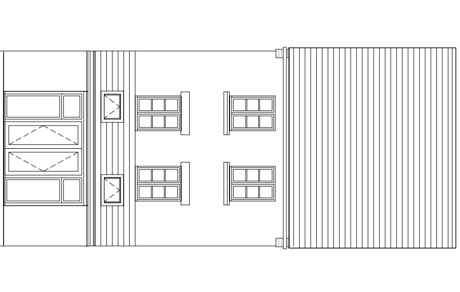
REAR ELEVATION
