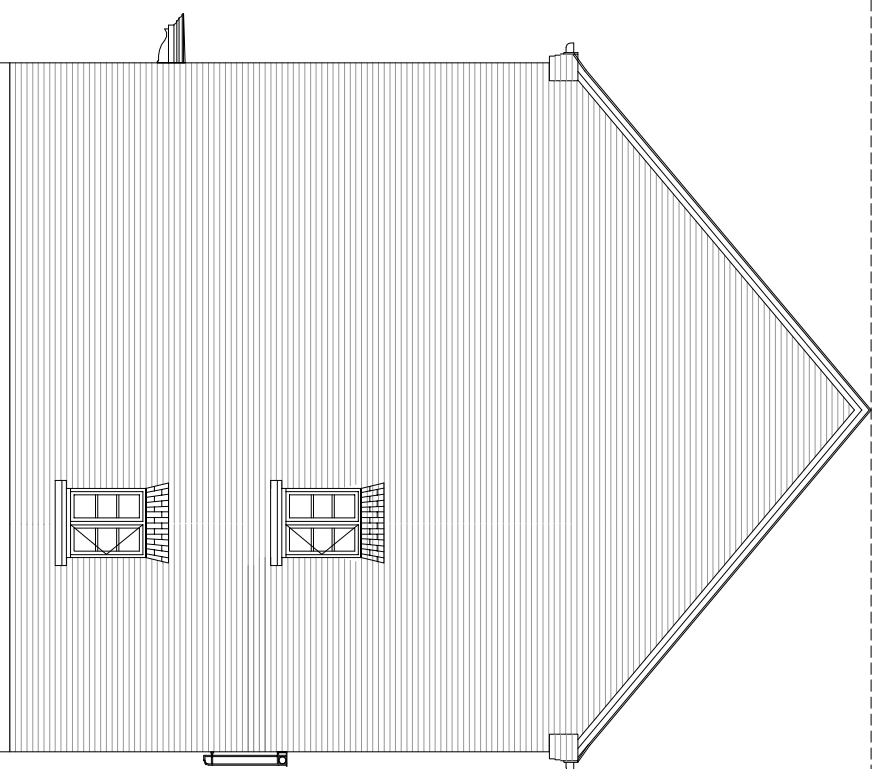
EOT ELEVATION (B)
