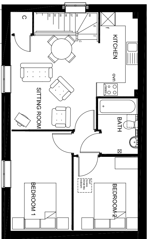
FIRST FLOOR PLAN PLOT 134 ONLY
