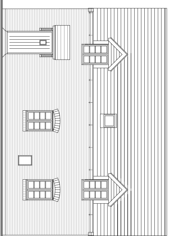
COURT ELEVATION
