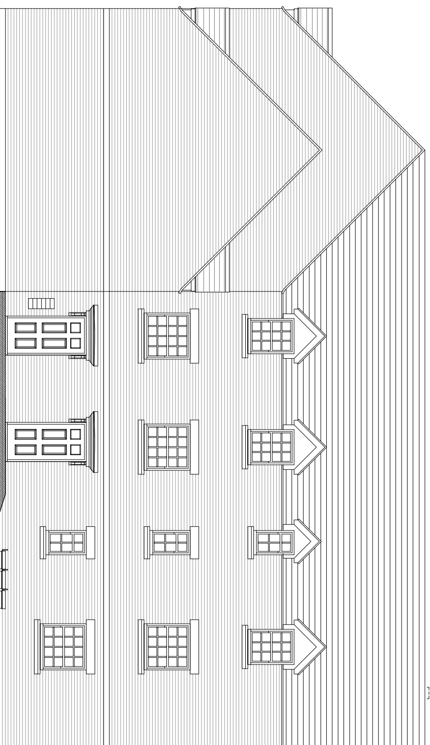
COURTYARD ELEVATION
