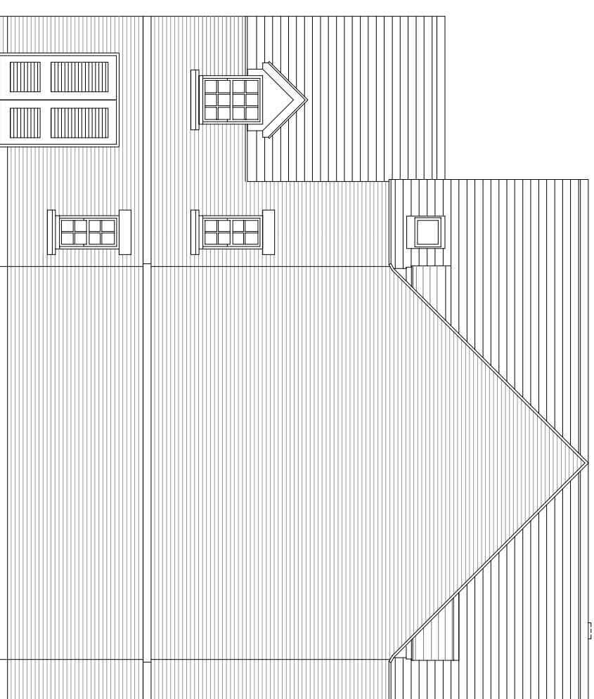
COURTYARD ELEVATION
