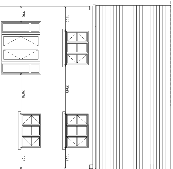
REAR ELEVATION
