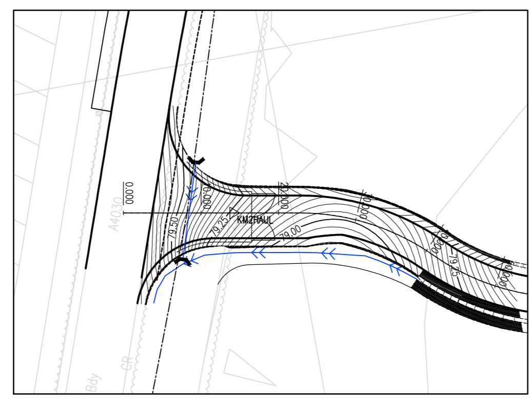
HAUL ROAD CONTOURS SCALE 1:500
