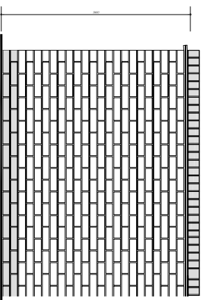
1800mm HIGH SCREEN WALL (STRETCHER BOND) Capping to be engineering brick on edge type FL or FH on Two courses plain tiles laid to fall to rear face with 45mm overhang and joints staggered.
