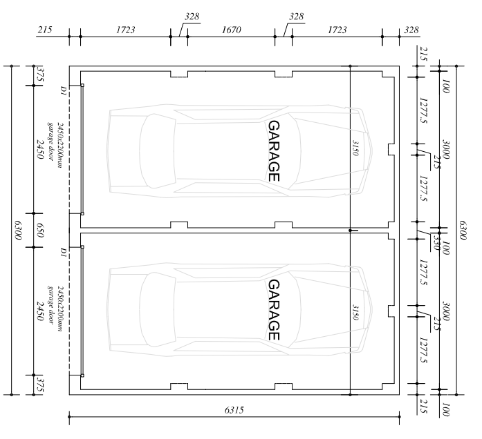
GARAGE - PLAN AGS2-2_1
