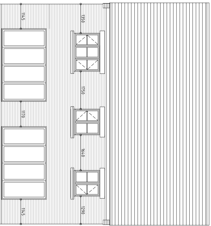
REAR ELEVATION
