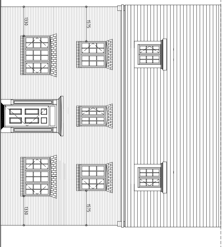
FRONT ELEVATION
