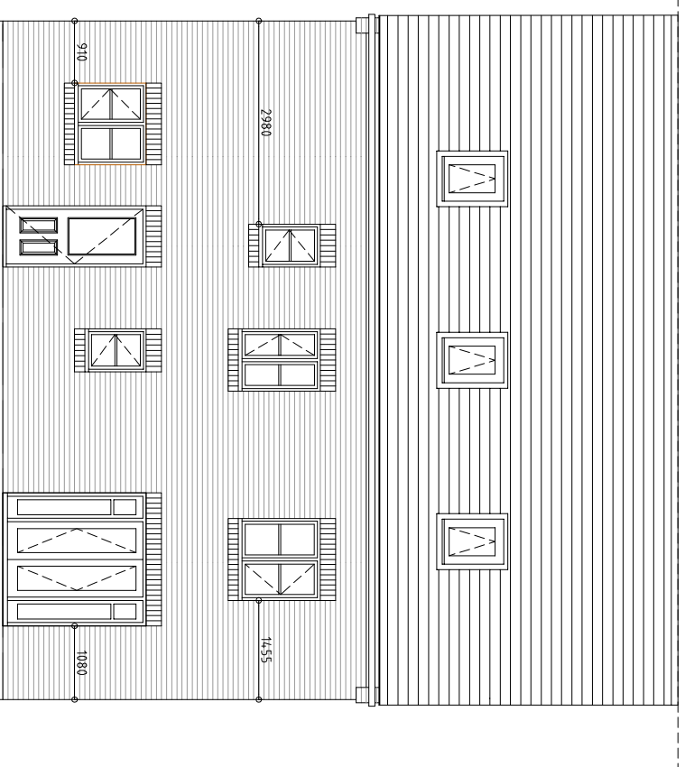
REAR ELEVATION
