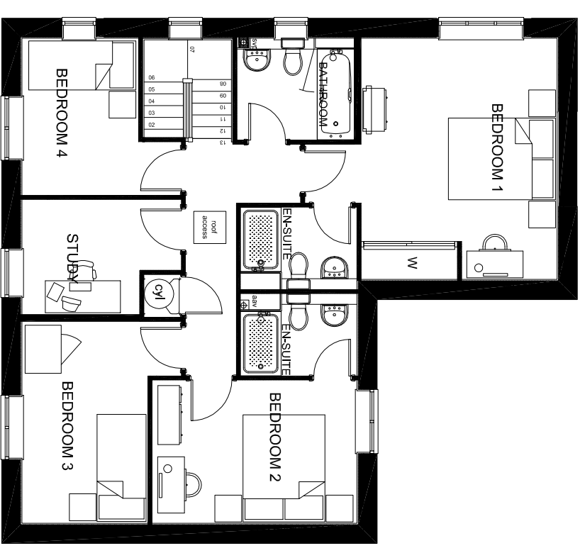
FIRST FLOOR ( PLOTS 22, 41, 104 & 201)
