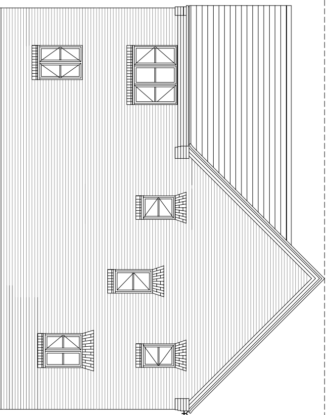
REAR ELEVATION
