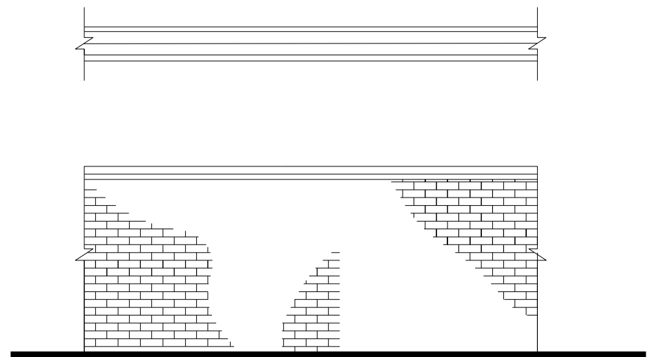
Plan and Elevation of Brick Wall 1:50
