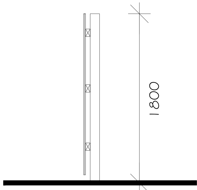
Typical Section 1:20
