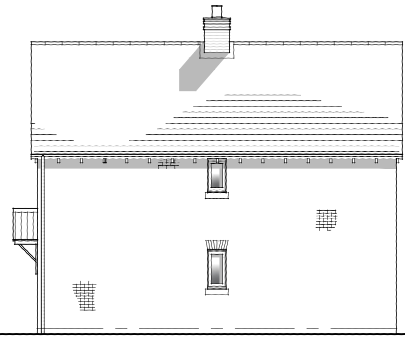
Plot 20 SIDE ELEVATION
