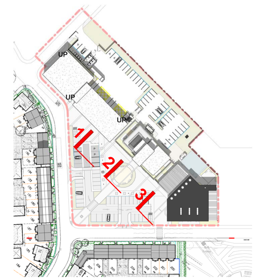
4 Key Plan Elevation Details 1 : 1250
