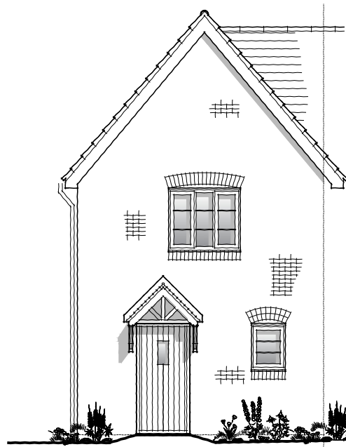
FRONT ELEVATION Plot 40, 43
