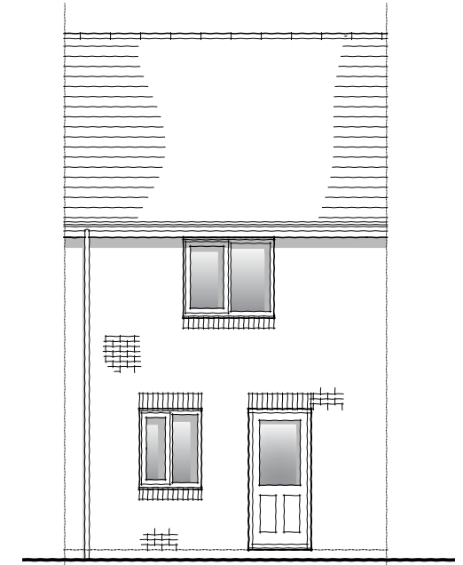
REAR ELEVATION Plots 37, 38, 39, 41, 42
