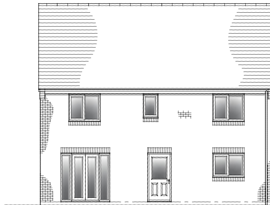
REAR ELEVATION
