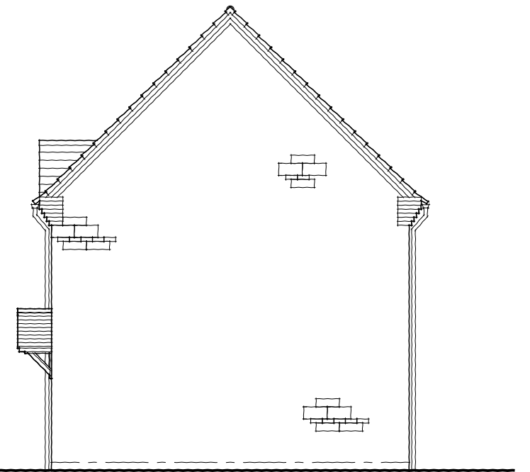
SIDE ELEVATION
