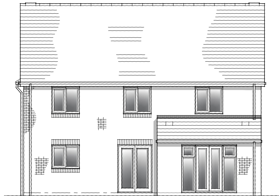
REAR ELEVATION
