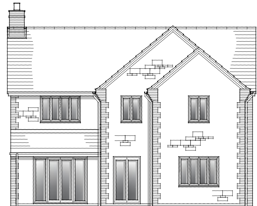
REAR ELEVATION
