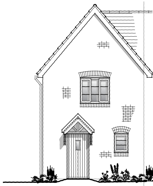
FRONT ELEVATION Plot 40, 43
