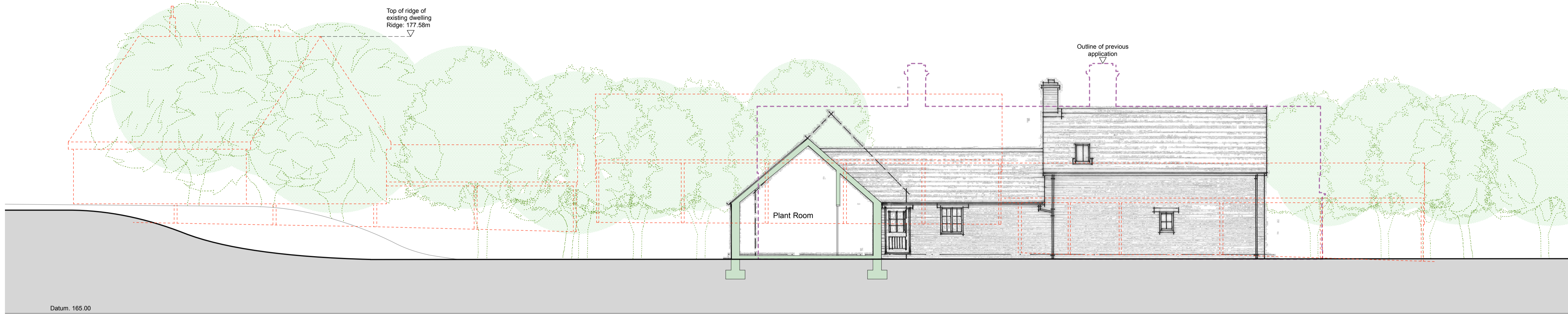
5: West Section and Elevation
