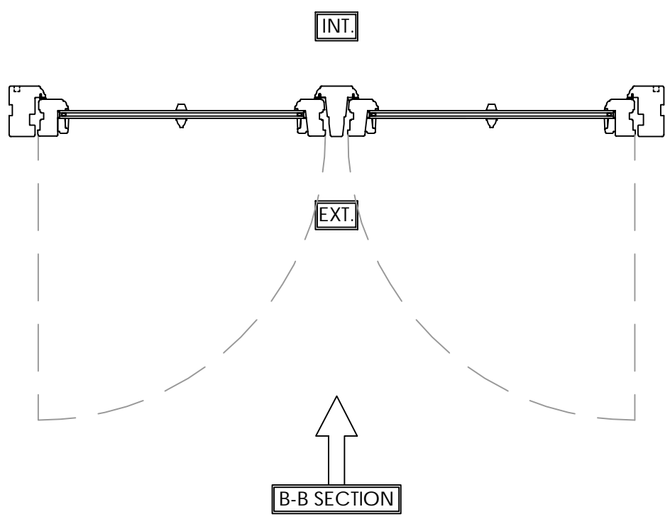
1. FRONT LOUNGE (14MM SLIMLINE GLAZING)
