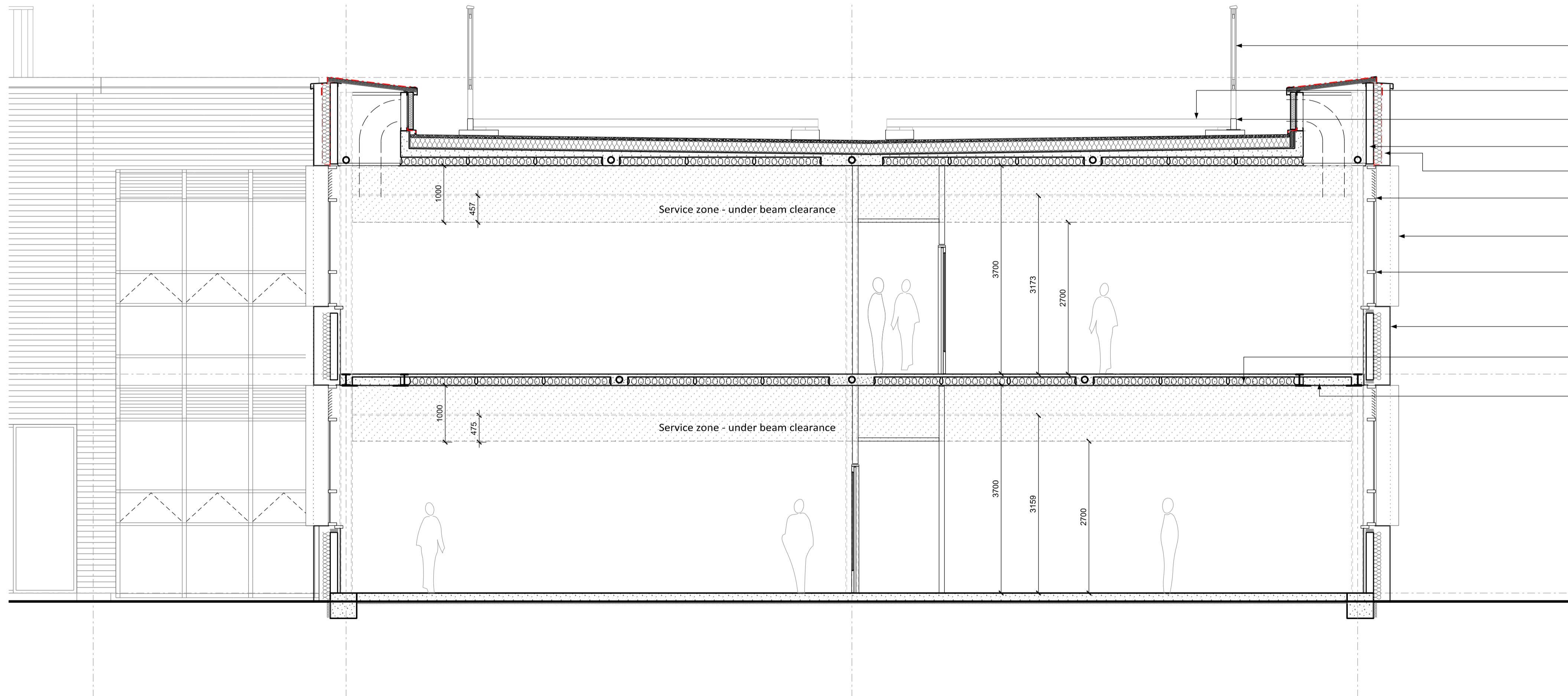
Proposed Section A-A 1:50 @ A1
