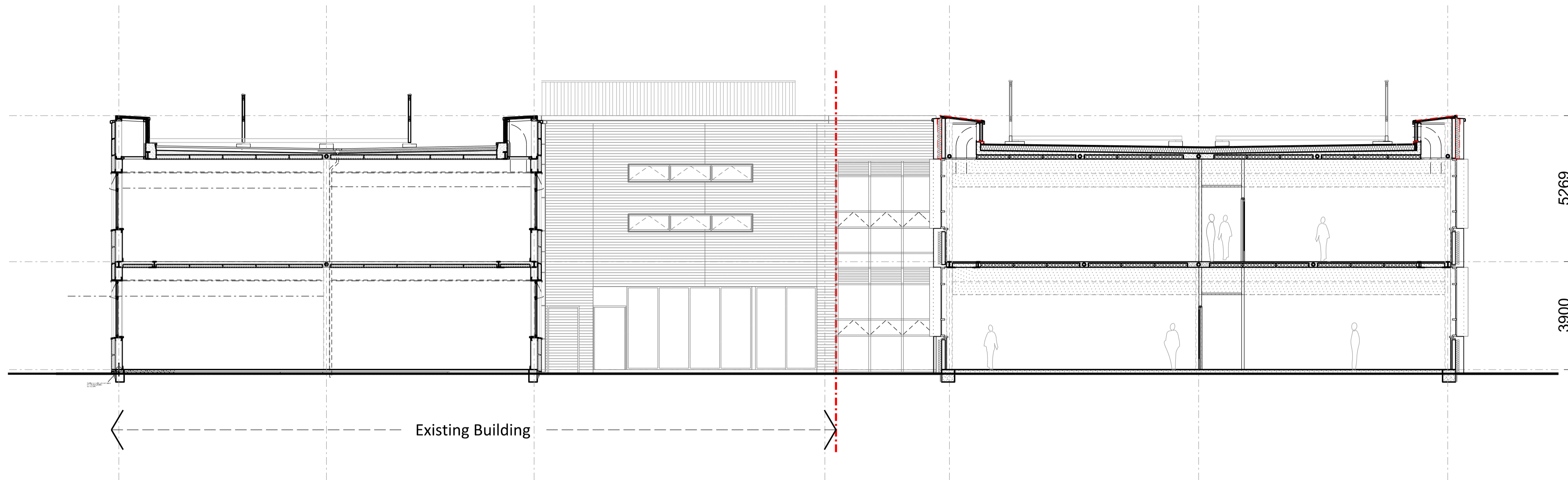
Proposed Section A-A 1:100 @ A1
