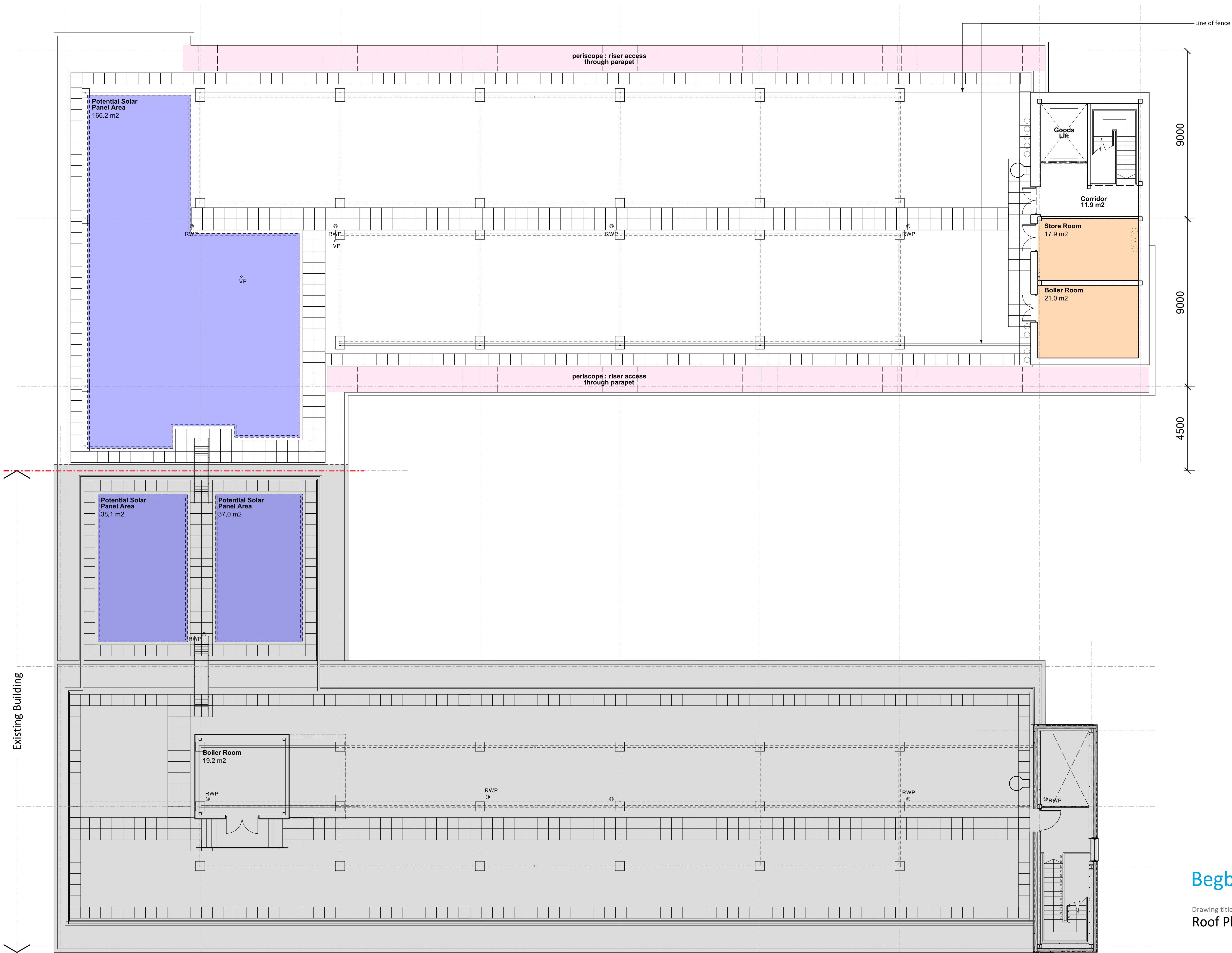
Upper Roof Plan
