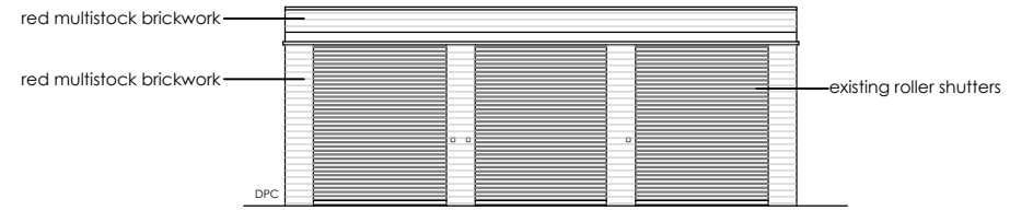
BUILDING 105 North Elevation - Existing
