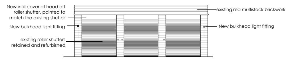
BUILDING 105 North Elevation - Proposed
