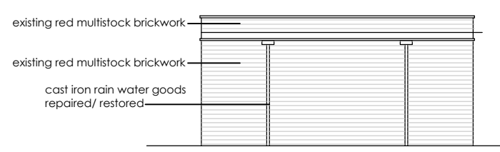
BUILDING 105 East Elevation - Proposed
