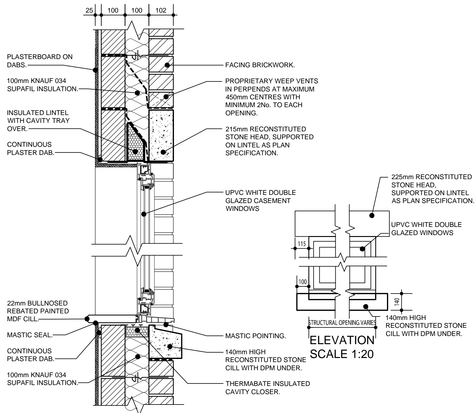
HEAD & CILL DETAILS SPLAYED HEADER
