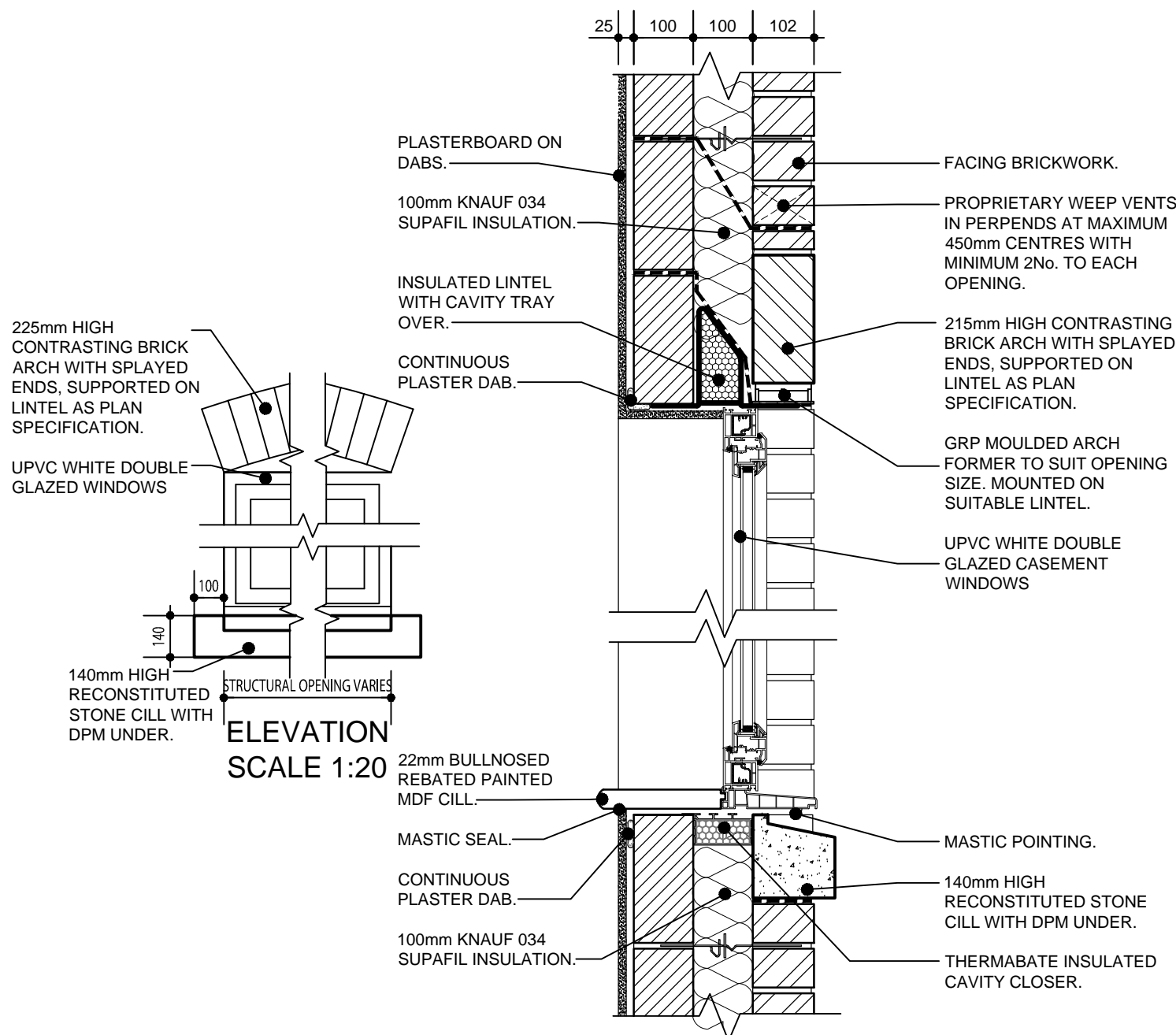
HEAD & CILL DETAILS ARCHED HEADER
