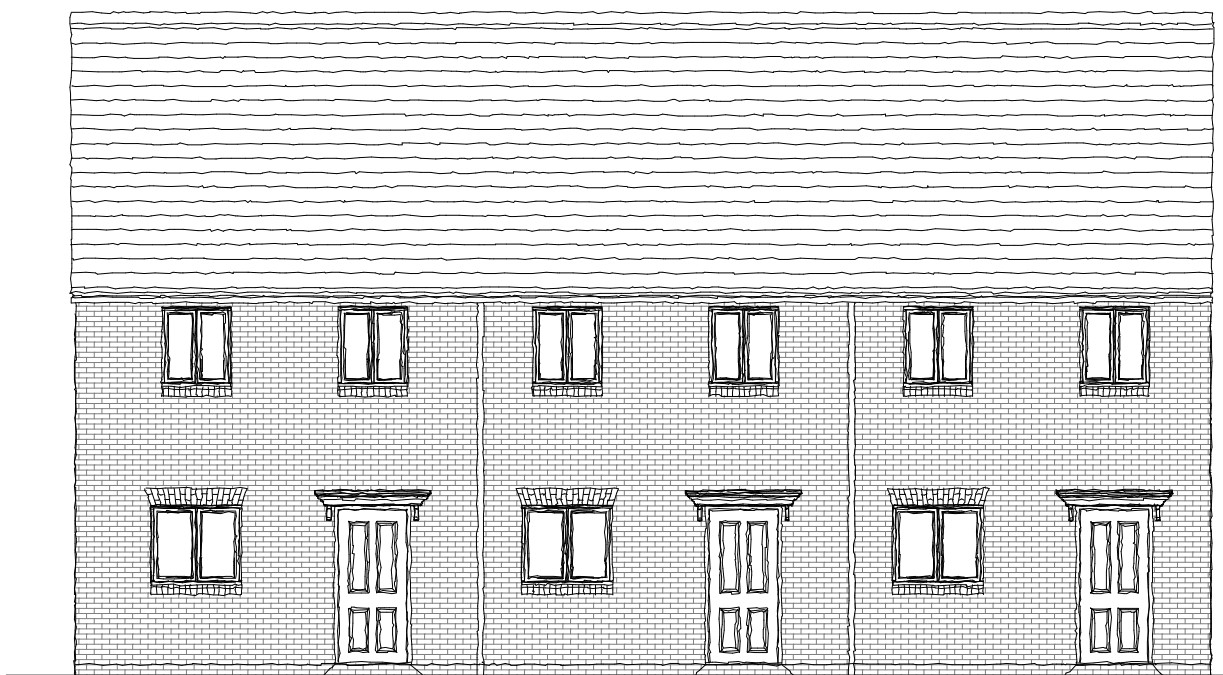
FRONT ELEVATION
