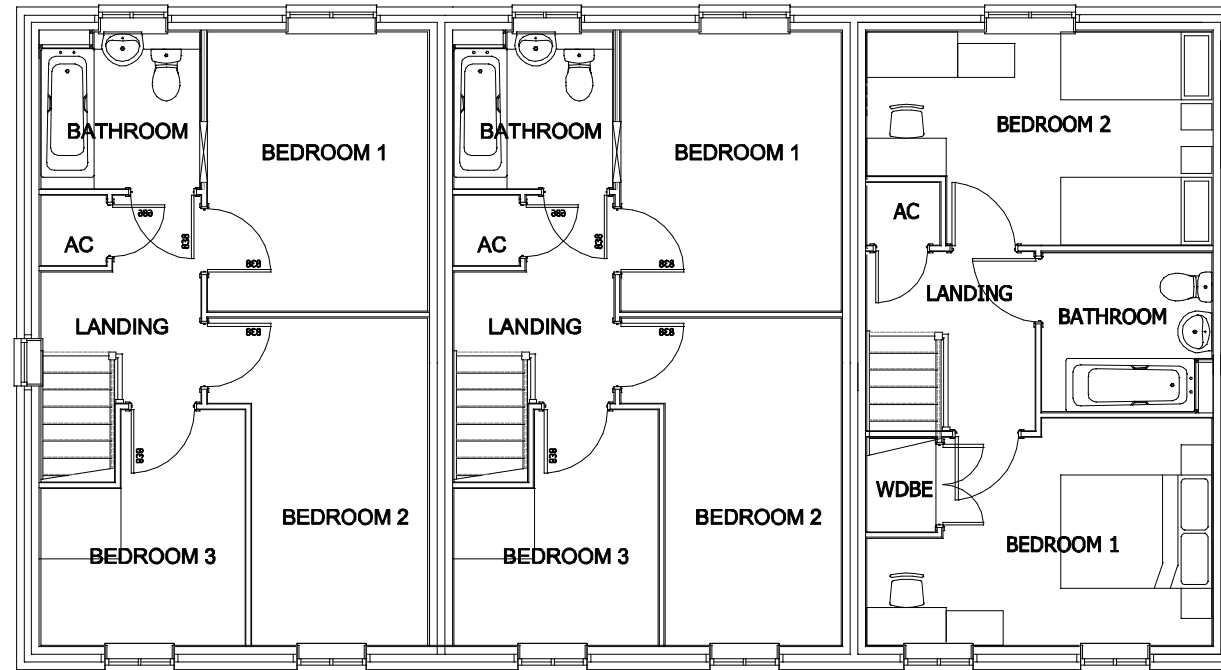
FIRST FLOOR
