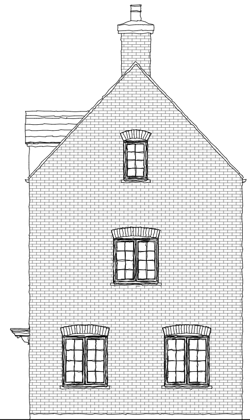
SIDE ELEVATION
