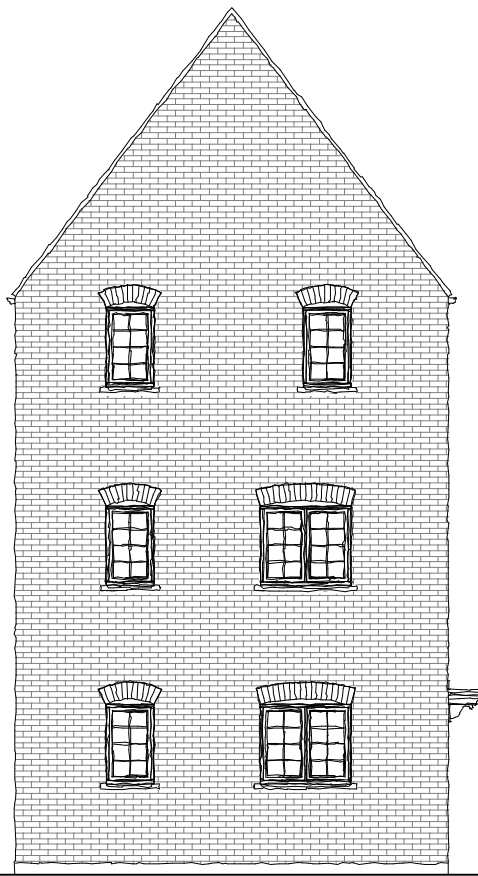
SIDE ELEVATION
