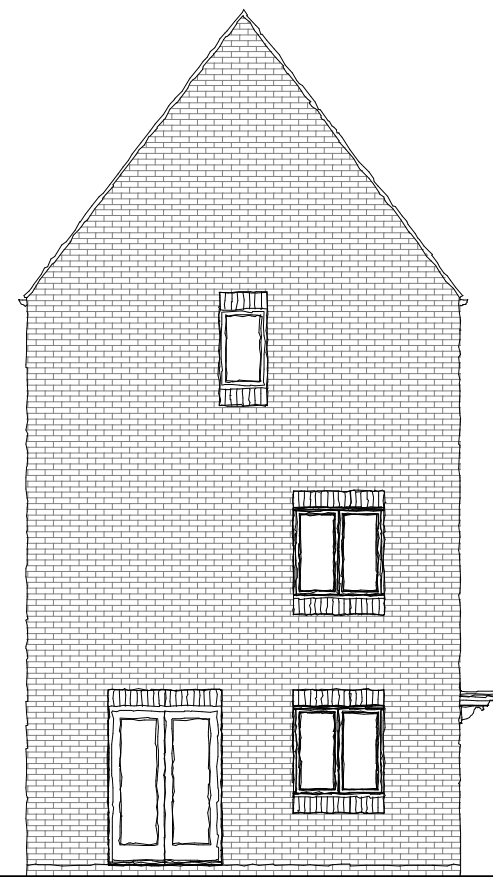
SIDE ELEVATION
