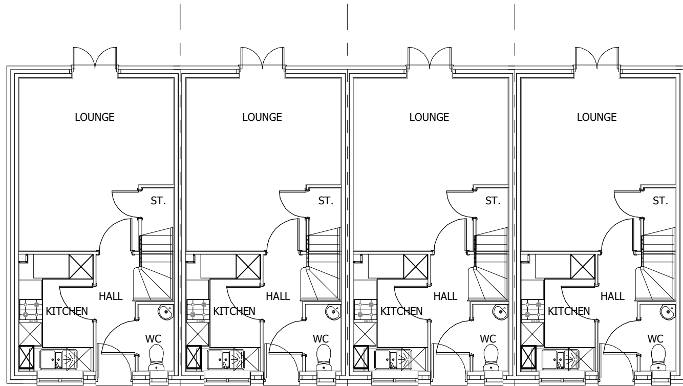
GROUND FLOOR
