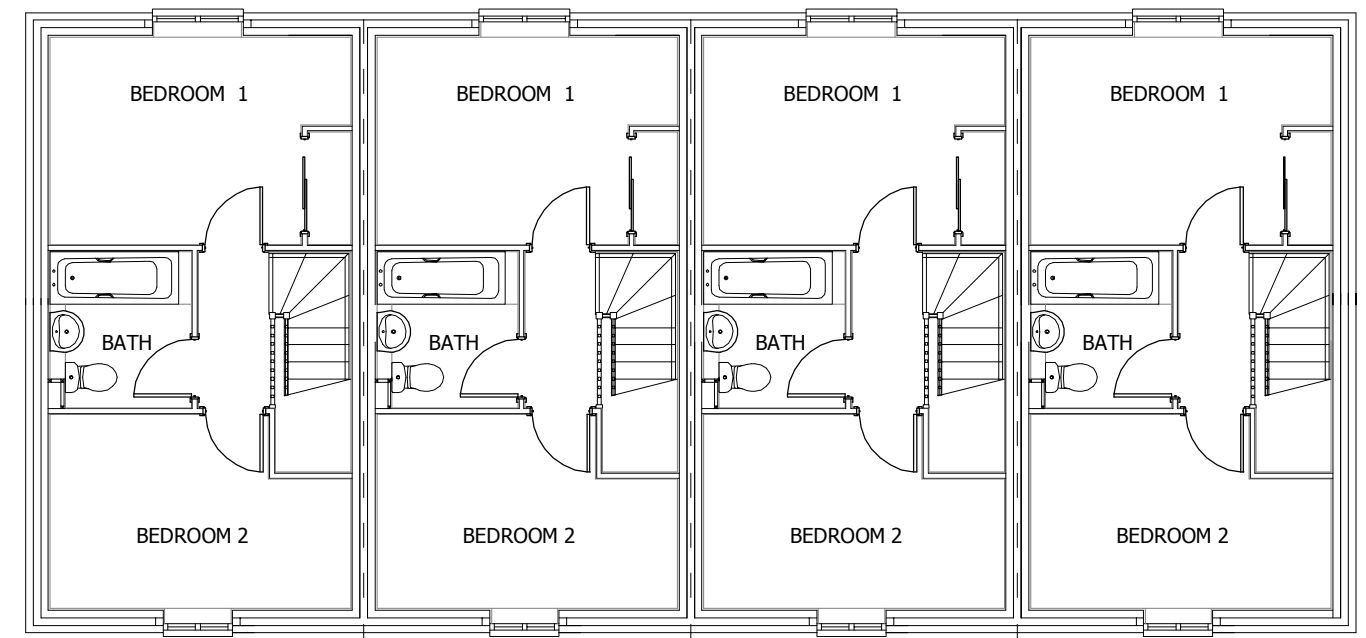
FIRST FLOOR
