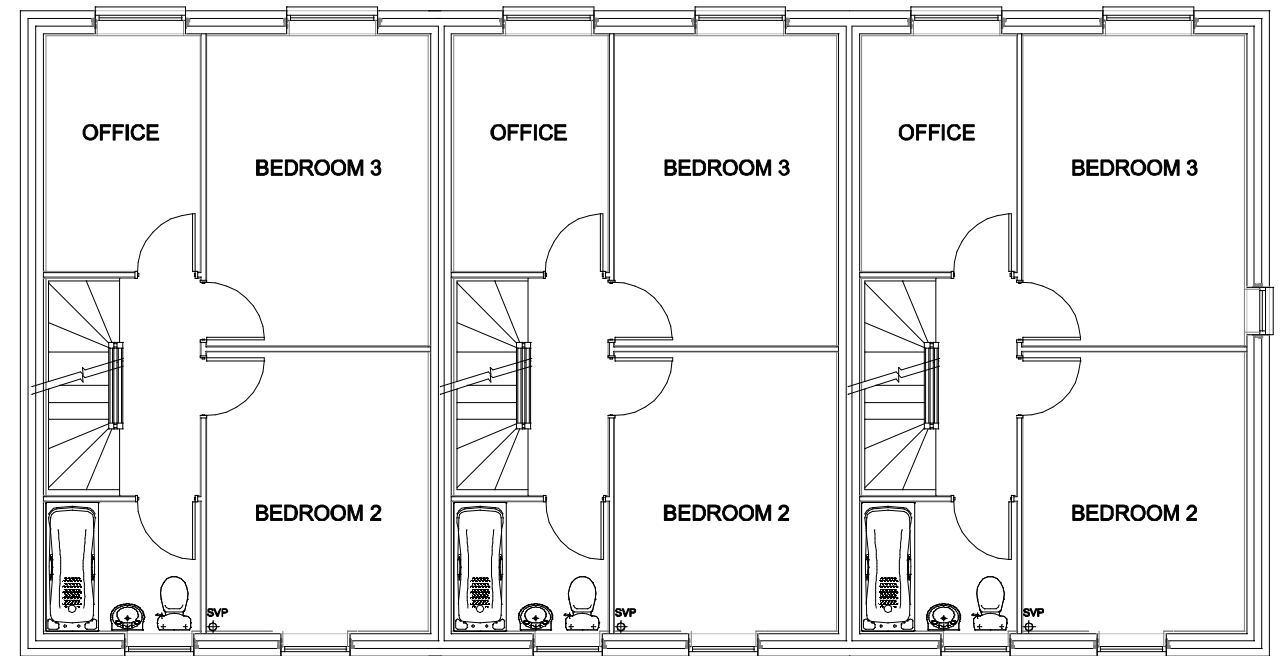
FIRST FLOOR
