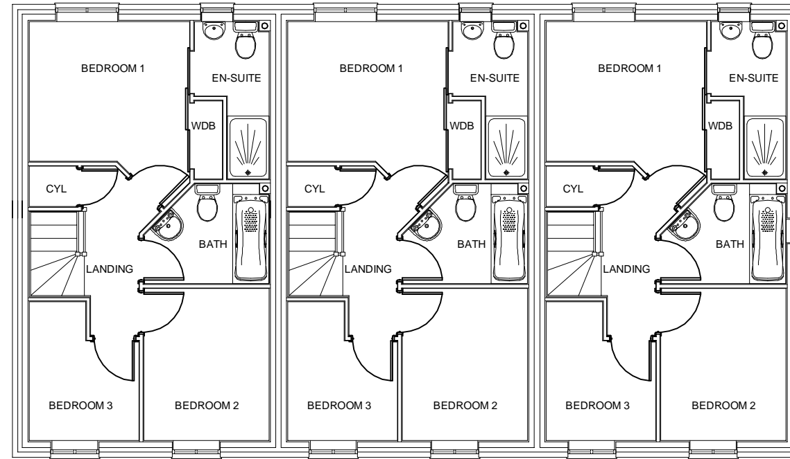
FIRST FLOOR
