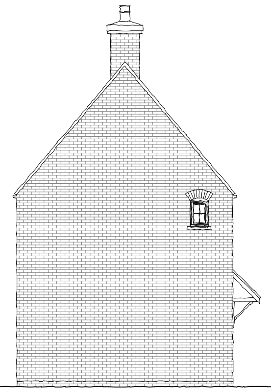
SIDE ELEVATION
