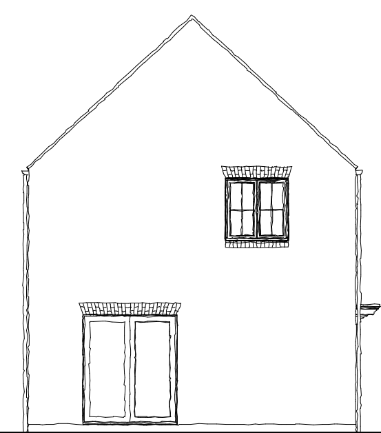
SIDE ELEVATION
