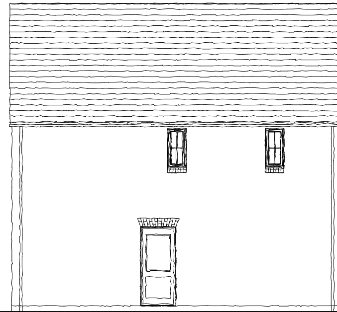
REAR ELEVATION
