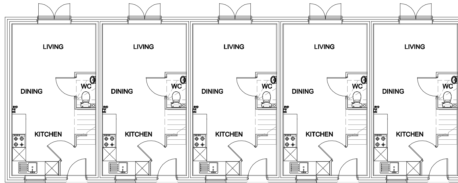
GROUND FLOOR
