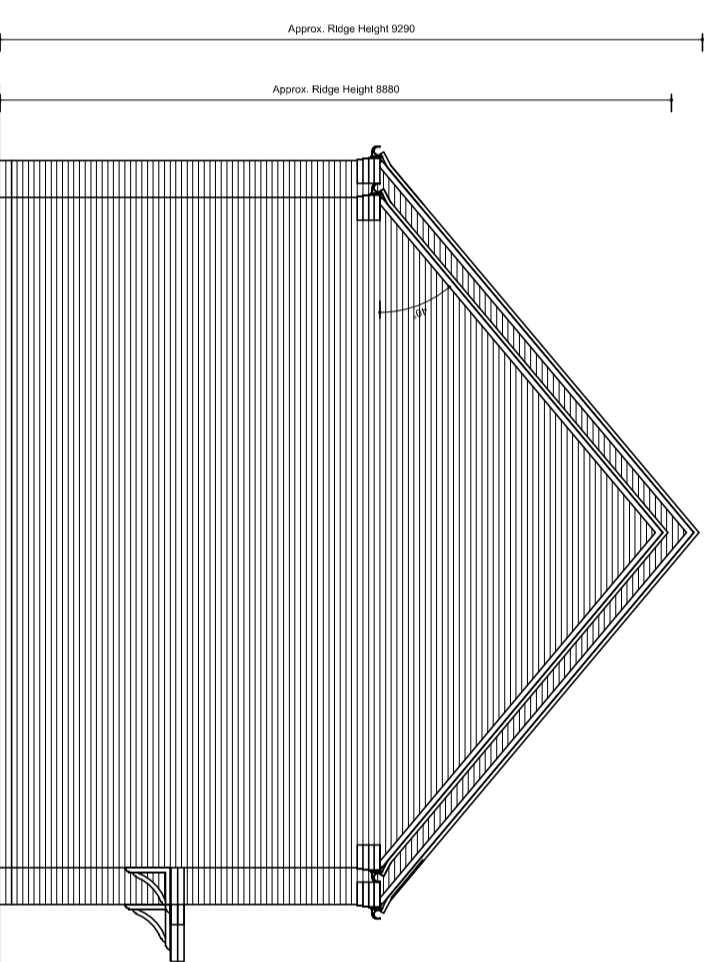
REAR ELEVATION
