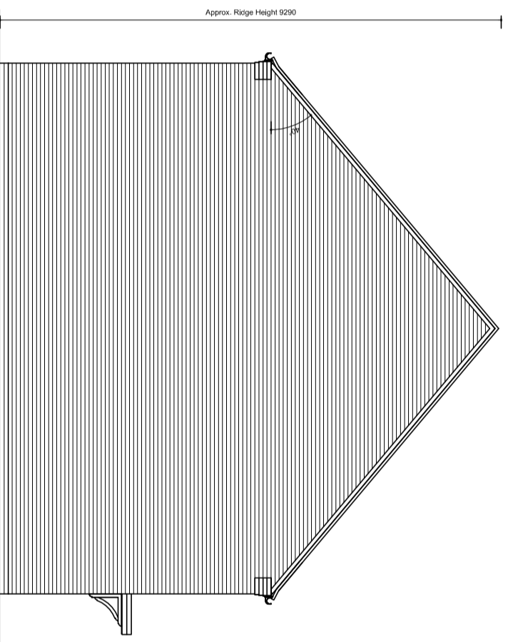
SIDE ELEVATION
