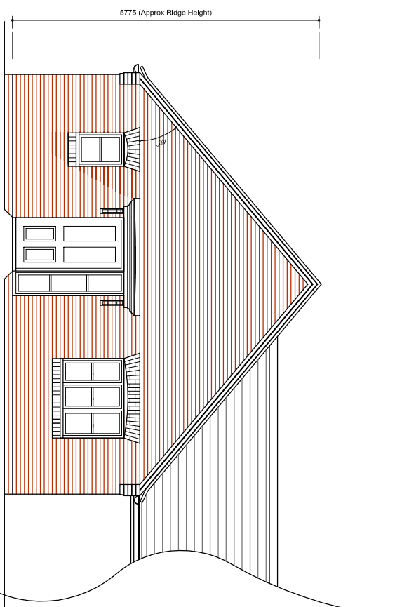
FRONT ELEVATION FORMAL TYPE K : SB2
