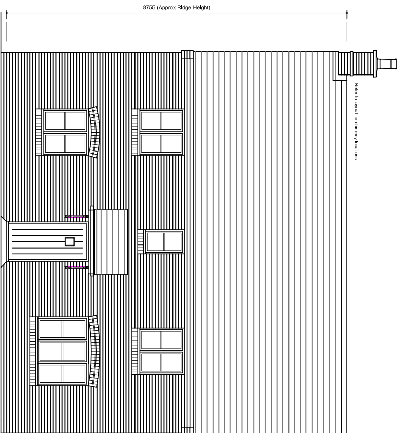
FRONT ELEVATION INFORMAL TYPE W : SW5006
