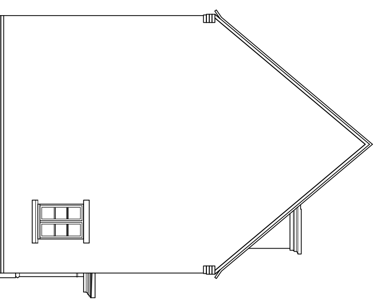
SIDE ELEVATION FORMAL TYPE I : P503
