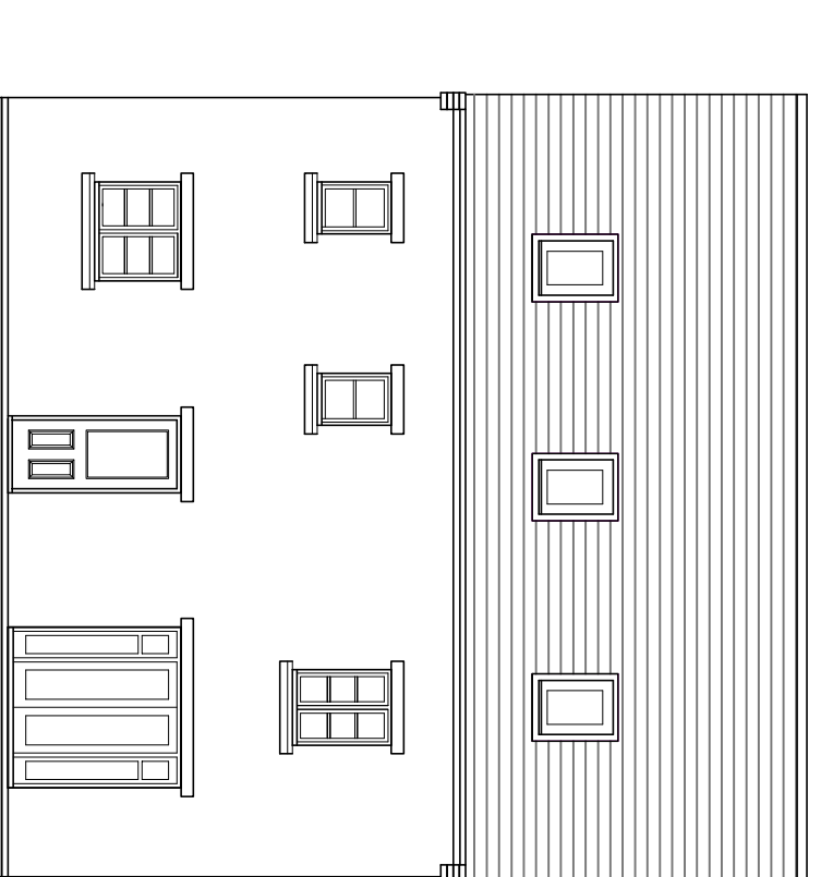
FRONT ELEVATION FORMAL TYPE I : P503
